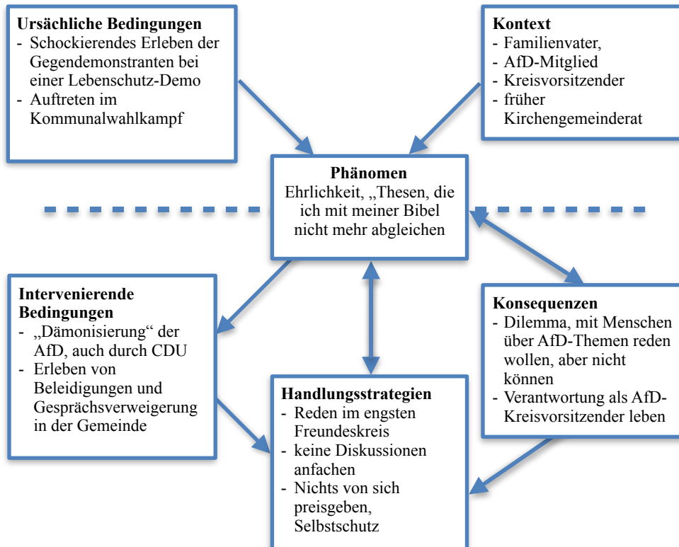
Abbildung 6: Kodierparadigma Peter
