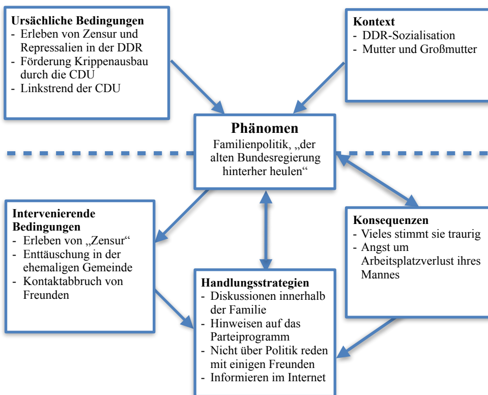
Abbildung 7: Kodierparadigma Anja
