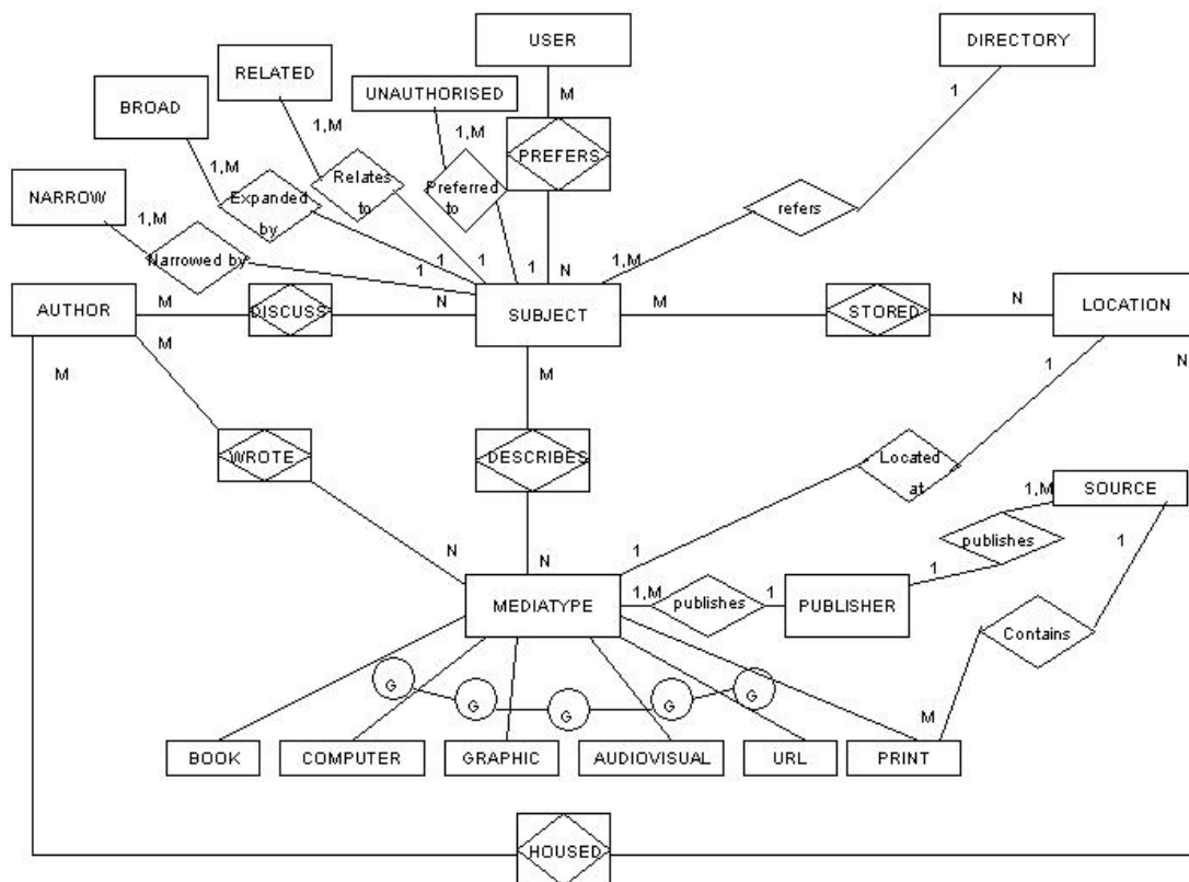
Figure 6.1 E-R diagram for rational therapy database
