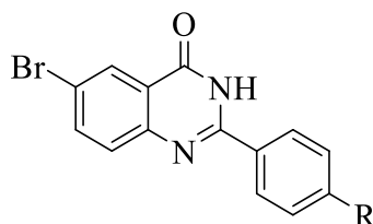
214a and 214b
