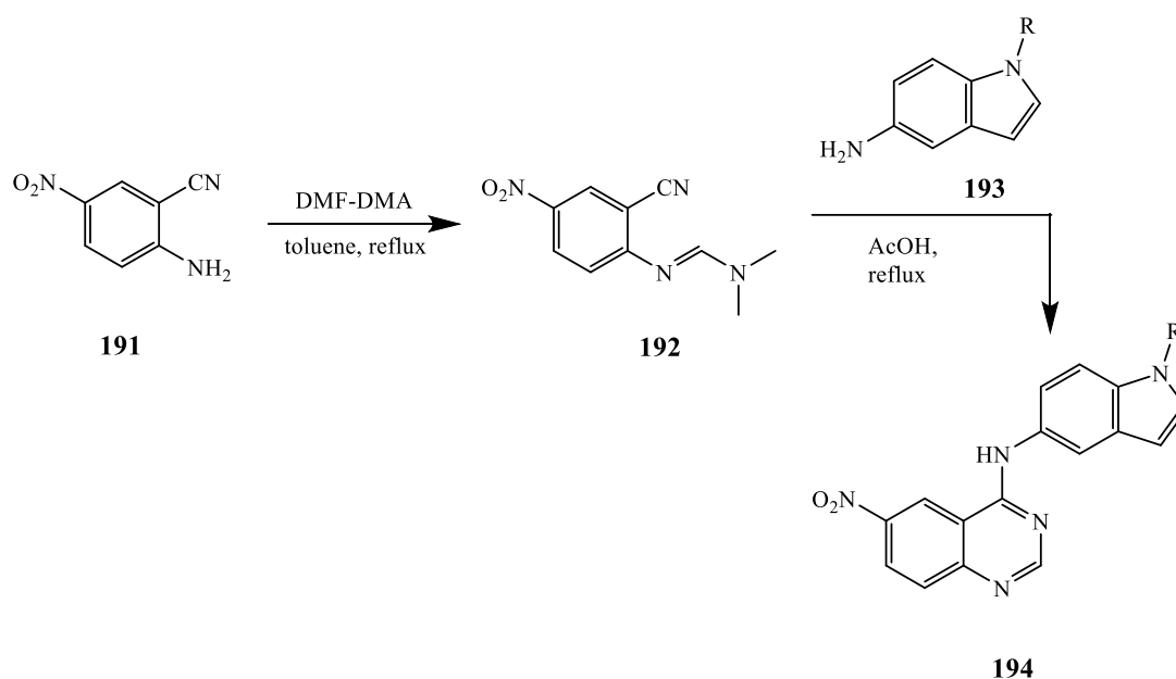
Scheme 54: Preparation of 194 from reaction of 192 with 193 .
