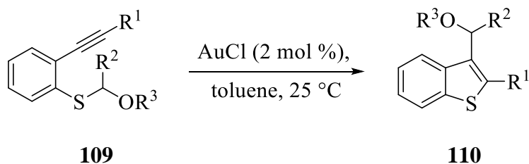
Scheme 30: Nakamura's gold-catalyzed cyclization of alkynyl thiophenols 109 .
