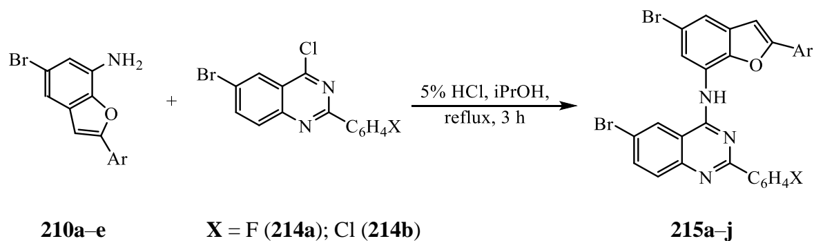
Scheme 67: Amination of 4-chloroquinazolines 214a, b with the 7-aminobenzofurans 210a–e
