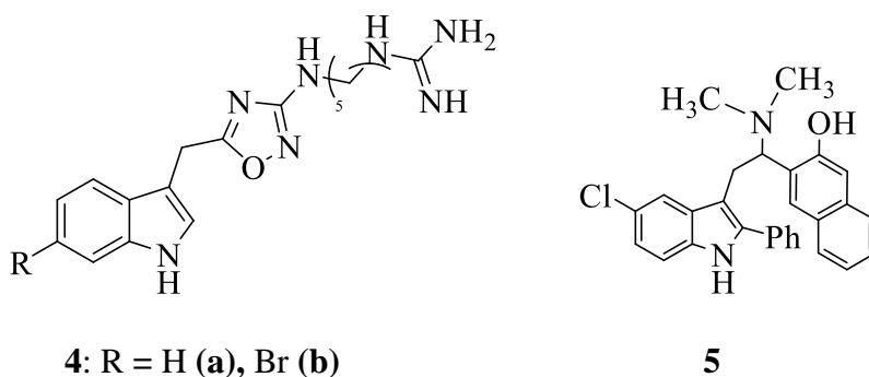
Figure 2: Examples of biologically active indole derivatives 4a , b and 5 .
