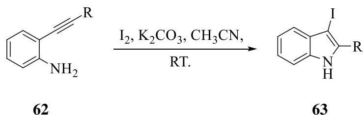
Scheme 12: I 2 -promoted cyclization of 62 to form 63 .
