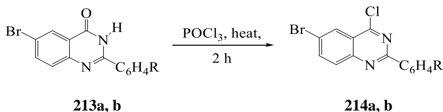
Scheme 66: POCl 3 -promoted aromatization of 213a, b .
