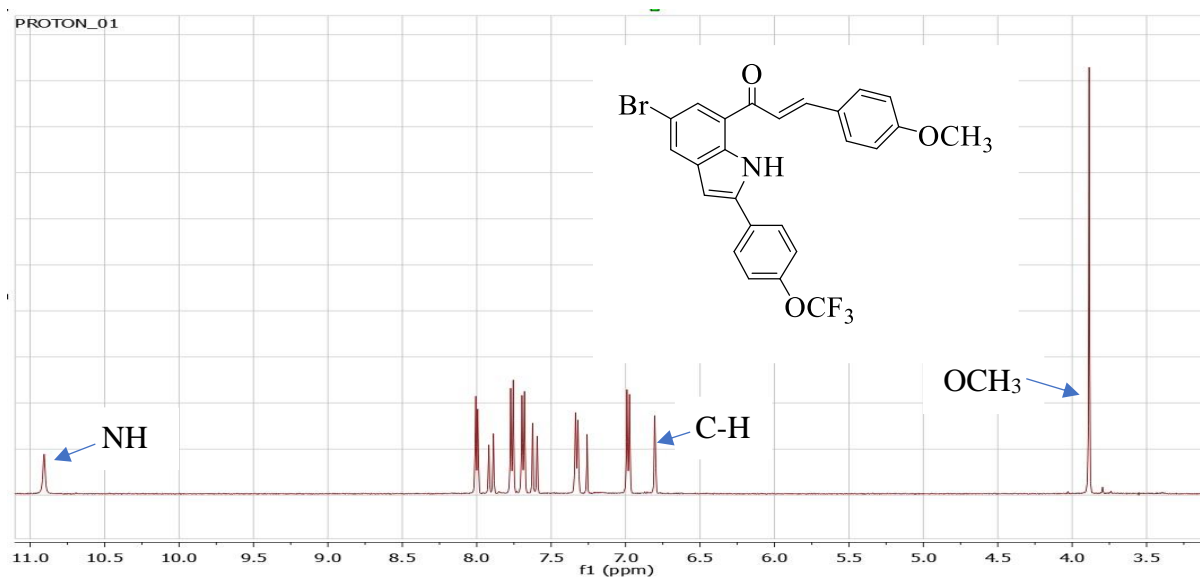
Figure 16: 1 H NMR spectrum of compound 201f in CDCl 3 at 500 MHz.
