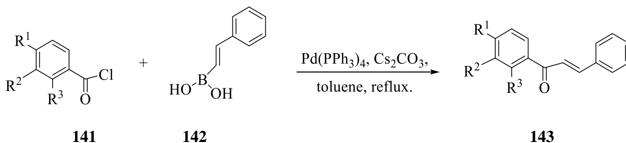
Scheme 39: Chalcone synthesis via Suzuki coupling.
