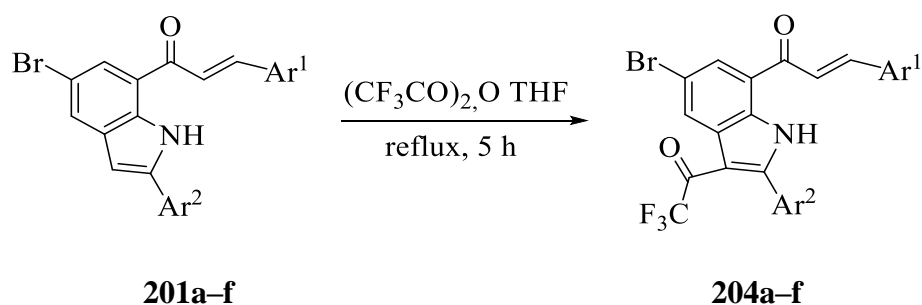
Scheme 61: TFAA-promoted C-3 acetylation of compounds 204a–f .
