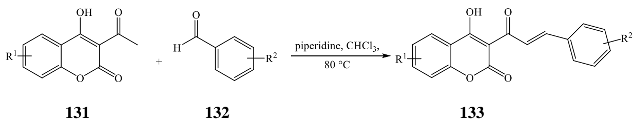
Scheme 36: Piperidine catalyzed synthesis of coumarinyl chalcones 133 .
