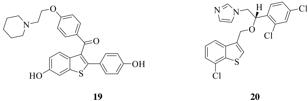
Figure 9: Examples of benzothiophene derivatives with medicinal applications.
