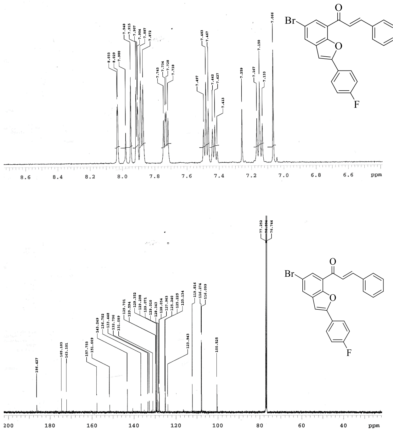
Figure 20: ^1\text{H} - and ^{13}\text{C} -NMR spectra of 203f in \text{CDCl}_3 at 500 and 125 MHz, respectively.
