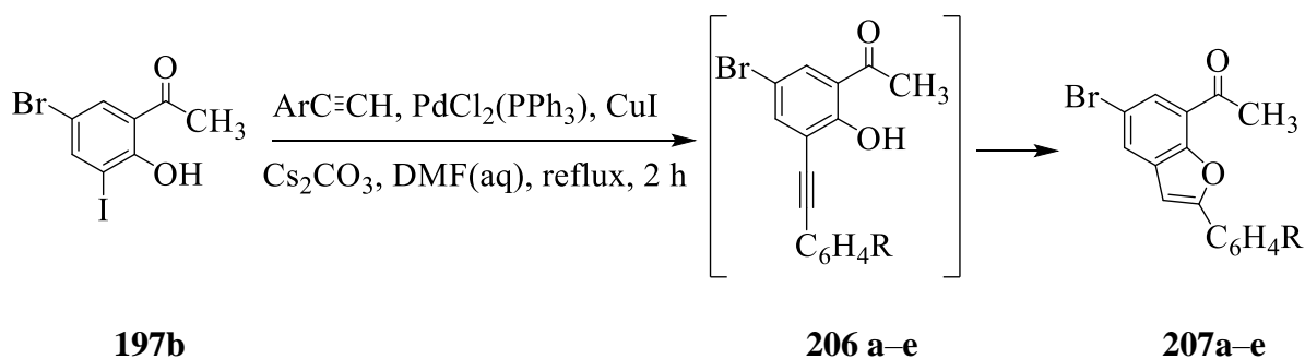
Scheme 63: Tandem Pd-catalysed Sonogashira cross-coupling and heteroannulation to afford 207a-e .
