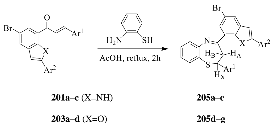
Scheme 62: Synthesis of benzothiazepines 205a–c and 205d–g .
