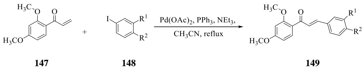
Scheme 41: Synthesis of chalcones 149 via intramolecular Heck cross coupling reaction.
