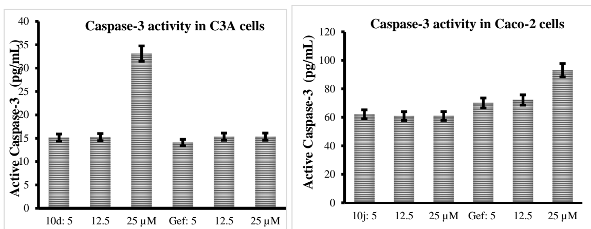
Figure 35: Effects of compounds 215d and 215j on Human Caspase-3 (Asp175) activity in C3A and Caco-2 cells against Gefitinib (Gef), respectively.
