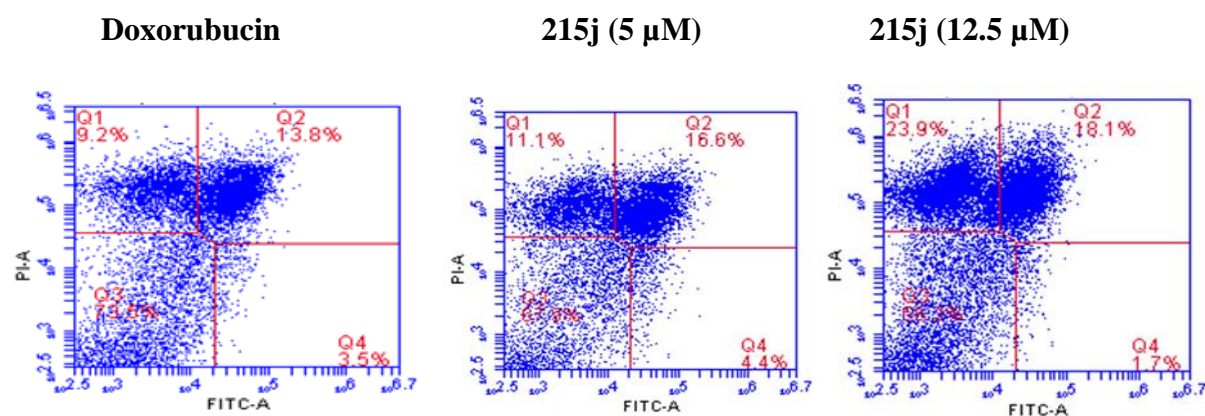
Figure 34: Effects of compounds 215d and 215j on the induction of apoptosis in C3A (a) and Caco-2 cells (b) as determined by Annexin V/PI staining. Data represent the percentage of apoptotic cells for the control and compounds 215d and 215j at 5 and 12.5 \mu\text{M} after 24 h.
