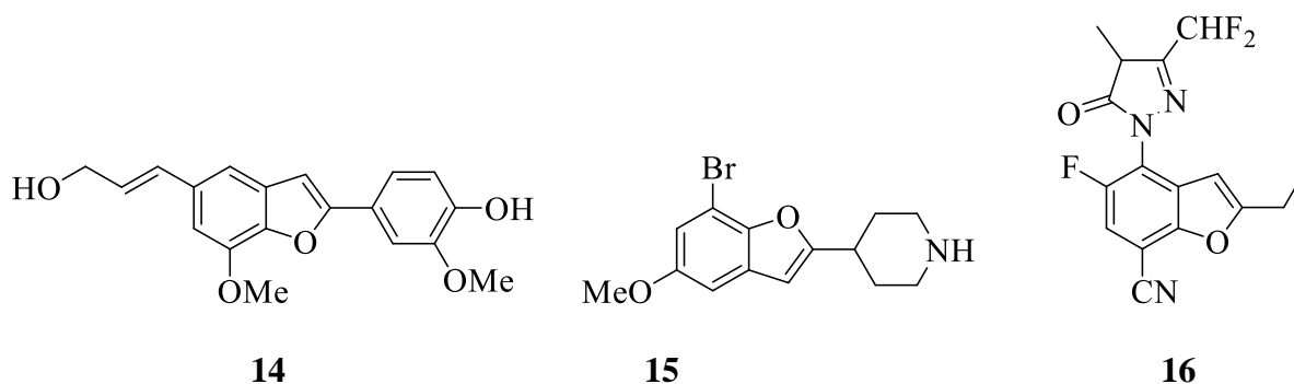
Figure 7: Examples of benzofurans with applications.
