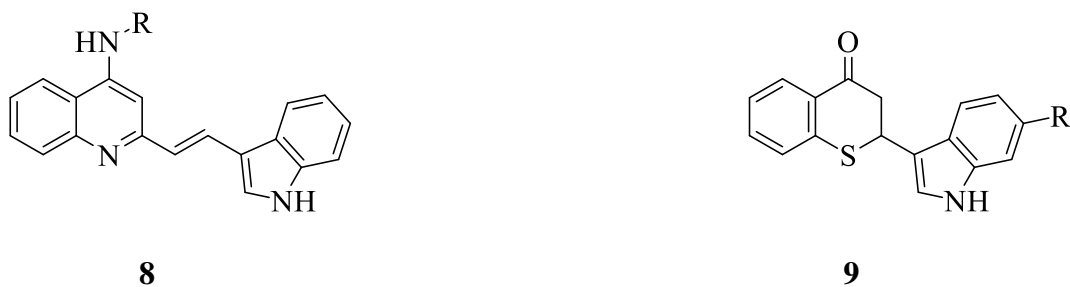
Figure 4: Example of indole-based quinolines 8 and thiaflavanone 9 of medicinal importance
