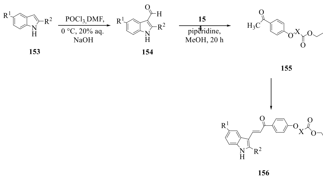
Scheme 43: Synthesis of indole-chalcones 156 .
