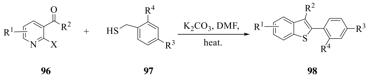
Scheme 26: K_2CO_3 -promoted cyclization of 96 to afford 98 .
