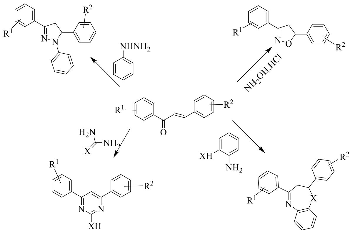
Scheme 49: Examples of reactions of chalcones with binucleophiles.
