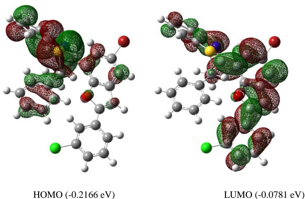
Figure 28. Frontier molecular orbitals of 205f using the B3LYP/6-311++G(d,p) basis set.
