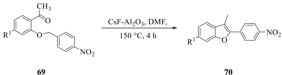
Scheme 15: CsF-Al 2 O 3 mediated cyclization of 2-arylalkoxy ketone 69 .
