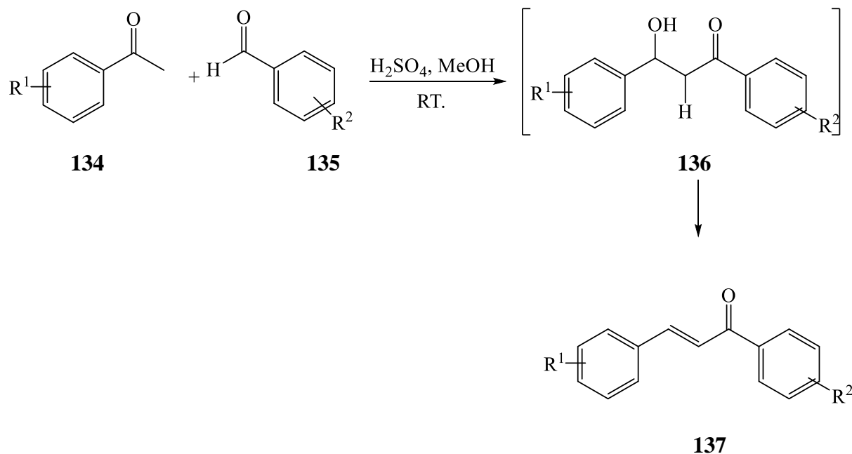
Scheme 37: Sulphuric acid catalyzed Claisen-Schmidt condensation.
