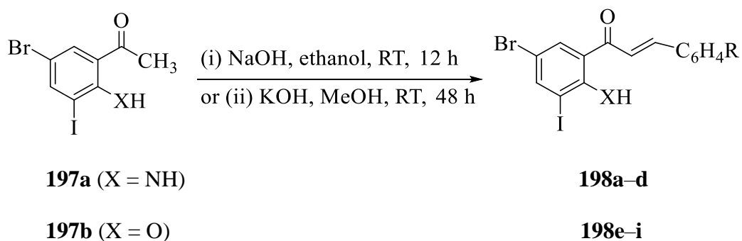
Scheme 57: Condensation of 197 (X = NH 2 or OH) with benzaldehyde derivatives.
