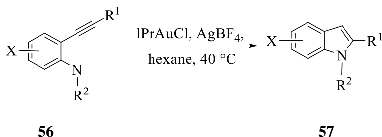
Scheme 10: IPrAuCl-catalysed cyclization of 56 to afford 57 .
