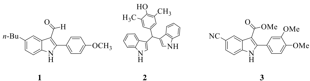
Figure 1: Examples of indoles with biological and photophysical properties.
