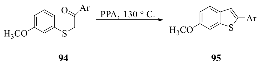
Scheme 25: PPA-promoted cyclization of 94 to afford 95 .
