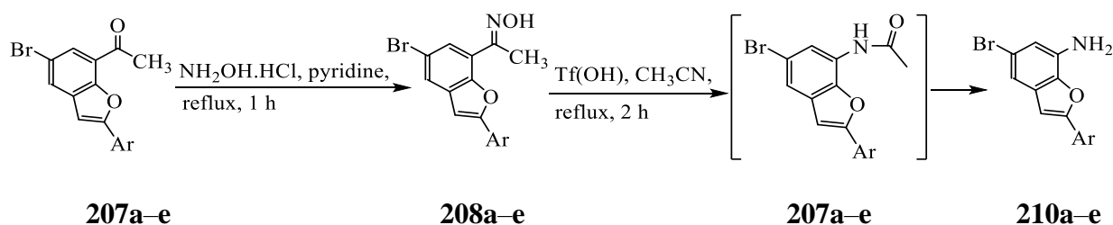
Scheme 64: One-pot Beckmann rearrangement and hydrolysis of oximes 208a–e into amines 210a–e .
