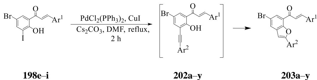
Scheme 60: Sonogashira cross-coupling of compounds 198e-i with terminal acetylenes.
