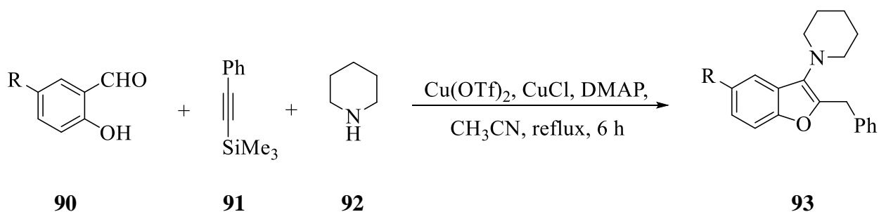
Scheme 24: Copper-catalyzed synthesis of substituted-benzofuran 93 .
