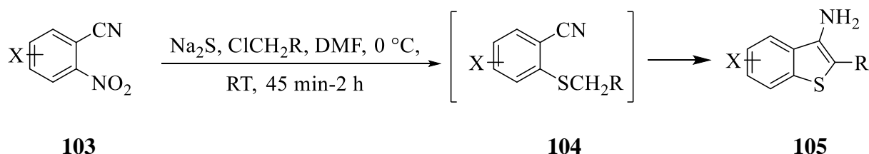
Scheme 28: Synthesis of benzo[ b ]thiophene derivatives 105 by Gewald reaction.
