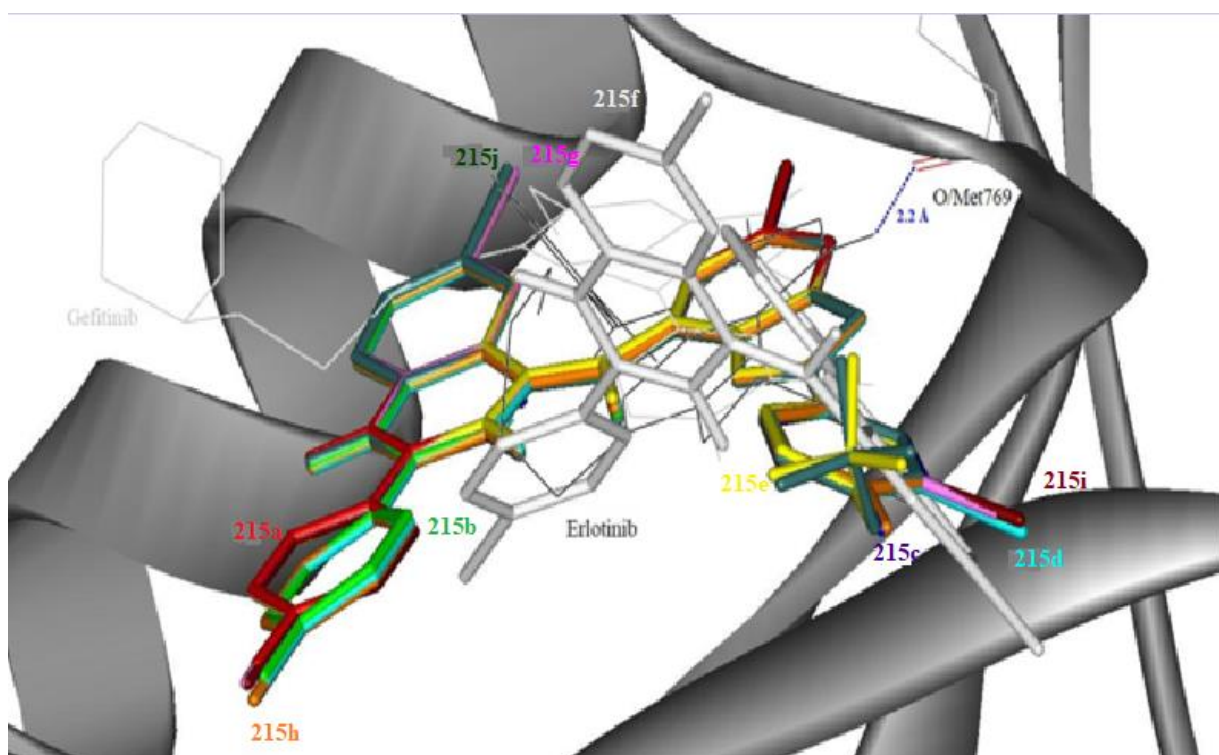
Figure 36: Docked conformation of Erlotinib (as docking control), Gefitinib and 4-aminoquinazoline-appended 2-arylbenzofurans (compound 215 ; stick representation) in the binding pocket of epidermal growth factor receptor (EGFR) kinase domain (surface and ribbon representation). Blue dotted lines are the direct hydrogen bonding formed between docked ligands and EGFR. The results for the synthesis and biological evaluation of the 4-aminoquinazoline-appended 2-arylbenzofurans have since been published. 173
