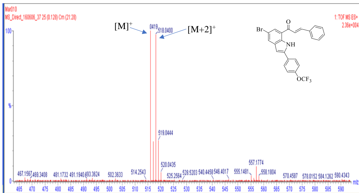
Figure 17: HR-MS of 201e using positive electrospray ionisation time-of-flight mass spectrometry.
