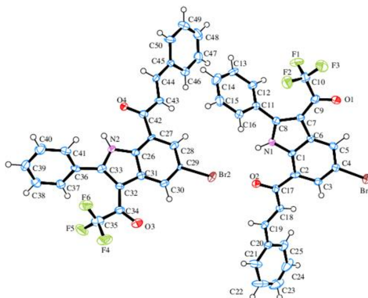
Figure 24: ORTEP diagram (50% probability level) of compound 204e
