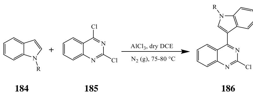
Scheme 52: Aluminium chloride-mediated cross-coupling of 184 with 185 to afford 186 .
