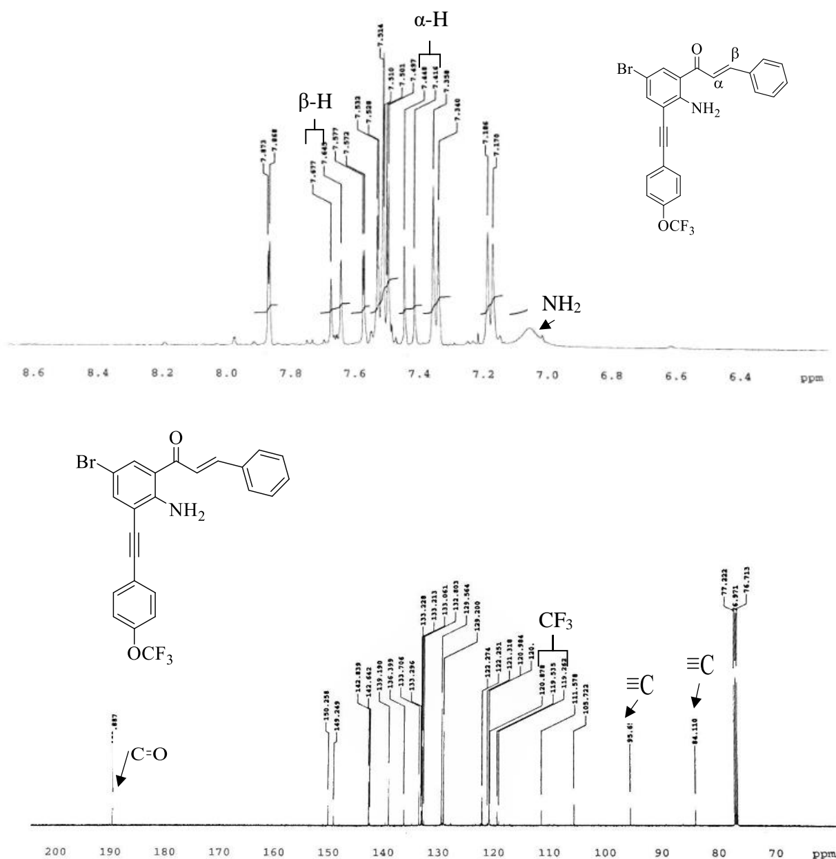
Figure 15: ^1\text{H} NMR spectrum of compound 200e in \text{CDCl}_3 at 500 MHz
