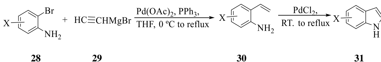
Scheme 2: PdCl 2 -catalysed heterocyclization of 30 to afford 31 .
