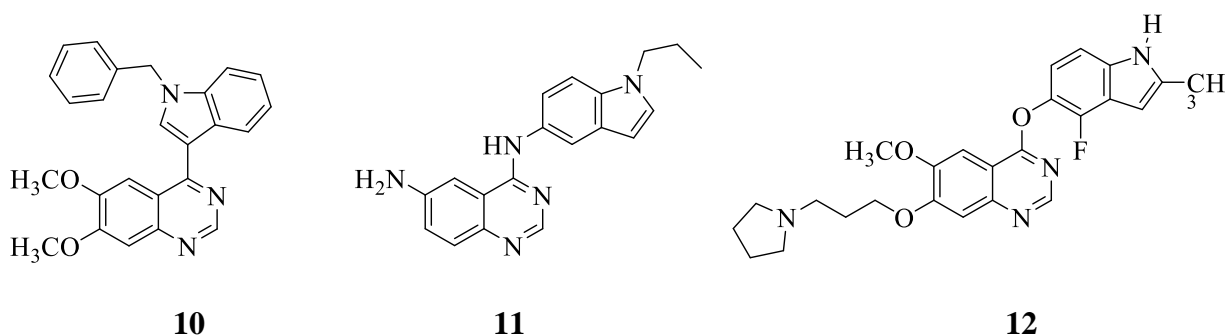
Figure 5: Examples of indole-appended quinazoline hybrids with biological properties
