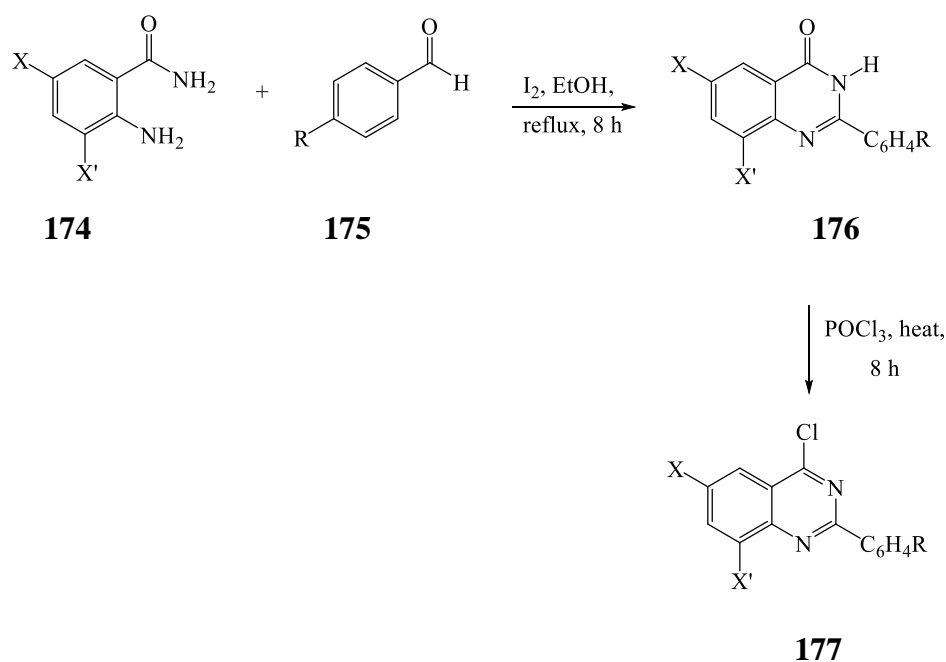
Scheme 50: Oxidative aromatization of quinazolin-4(3 H )-one
