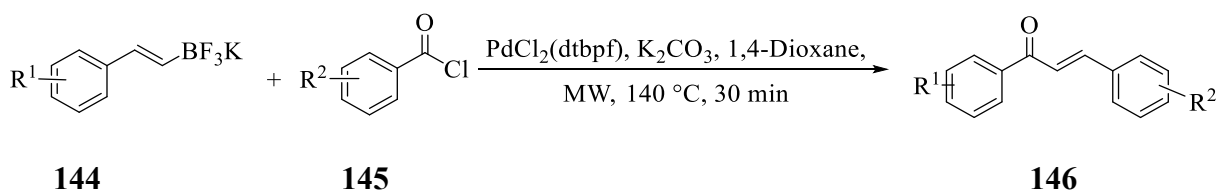
Scheme 40: Palladium catalysed Suzuki cross-coupling for the synthesis of chalcones 146 .
