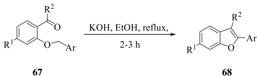
Scheme 14: Base mediated cyclization of 2-arylalkoxy ketones 67 .
