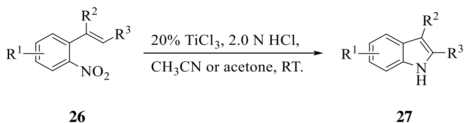
Scheme 1: Reductive cyclization of 26 to afford 27 .
