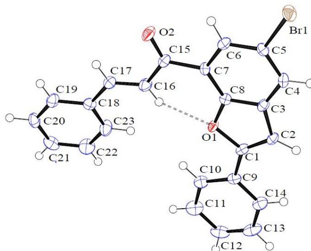
Figure 21: Oak Ridge Thermal Ellipsoid Plot (ORTEP) diagram of 203a . Displacement ellipsoids are drawn at the 50% probability level and H atoms are shown as small spheres of arbitrary radii
