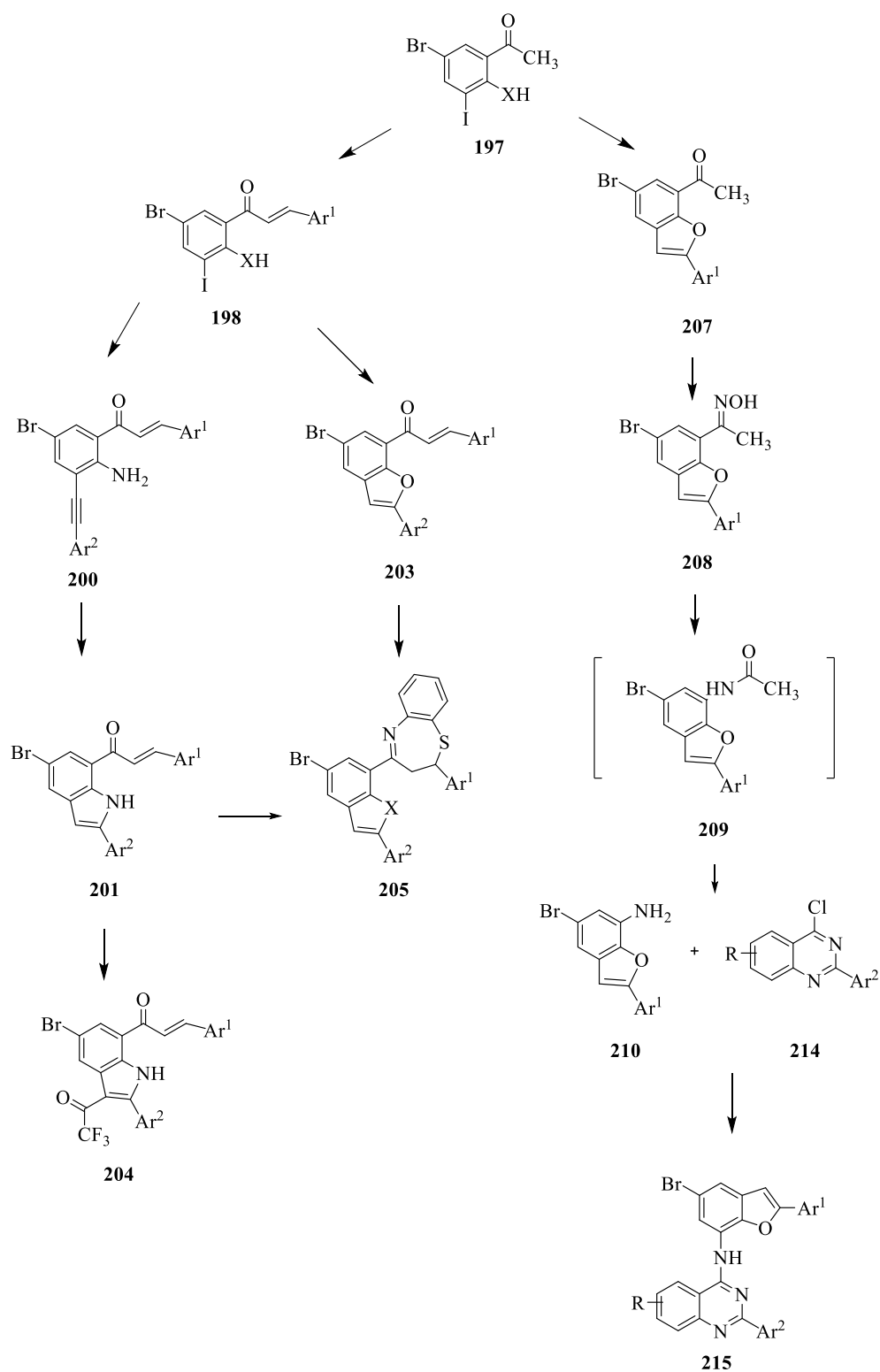
Figure 13: Generalized scheme depicting reaction pathways followed to prepare the compounds described in this investigation.
