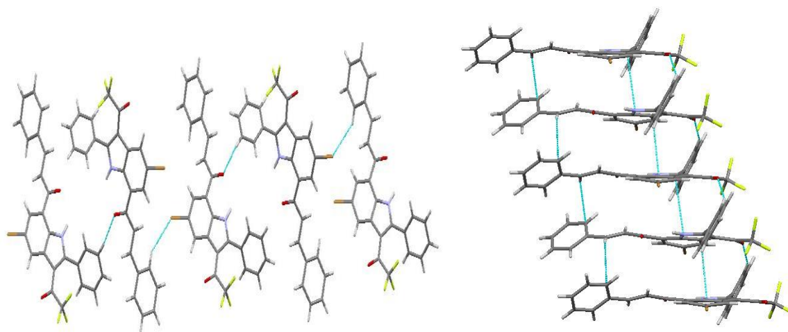
Figure 25: Packing diagram of compound 204e
