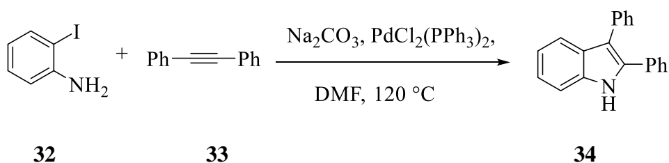
Scheme 3: Larock heteroannulation of 32 with 33 to afford 34 .
