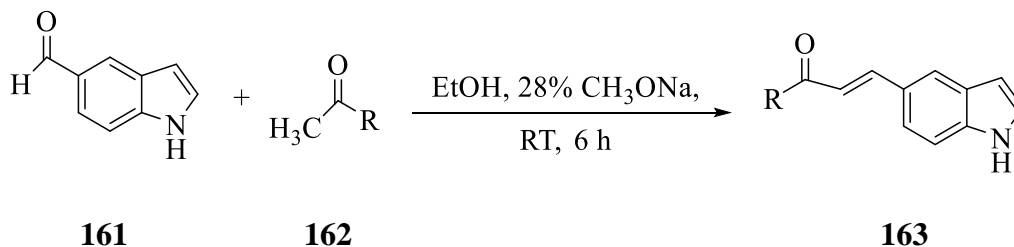
Scheme 45: Synthesis of indole-chalcones 163 .
