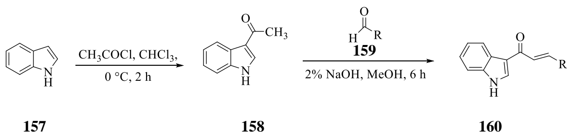
Scheme 44: Synthesis of indole-chalcones 160 .
