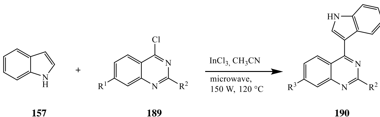
Scheme 53: Hybridization of 157 with 189 to afford 190 .
