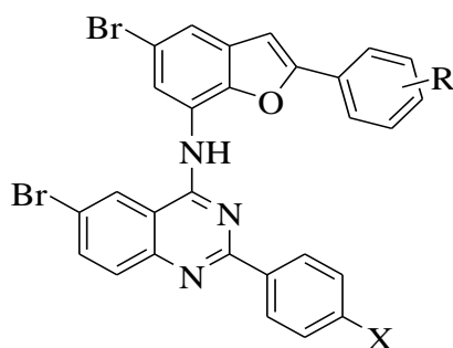
215a–e (X = F) & 215f–j (X = Cl)
