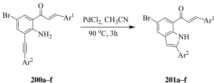
Scheme 59: Palladium chloride-mediated cyclization of 200a–f .
