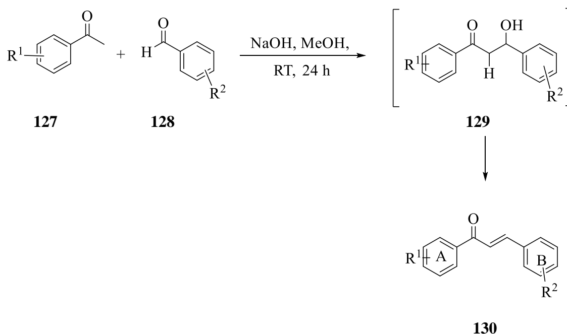
Scheme 35: Synthesis of substituted-chalcone 130 by Claisen-Schmidt condensation.
