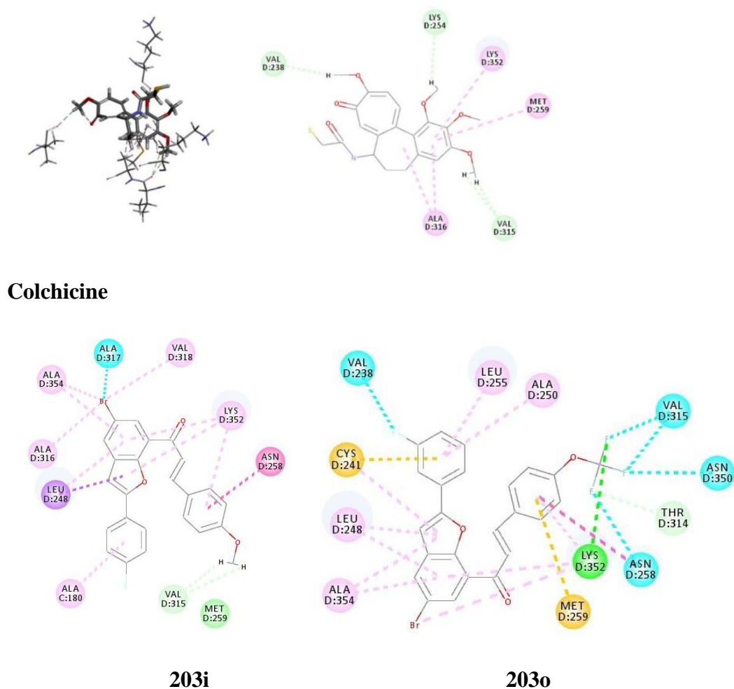
Figure 32. (a) 2D interaction diagrams for the binding of tubulin (PDB code: 1SAO) with colchicine, 203i and 203o . Residues are annotated with their three-letter amino acid code.
