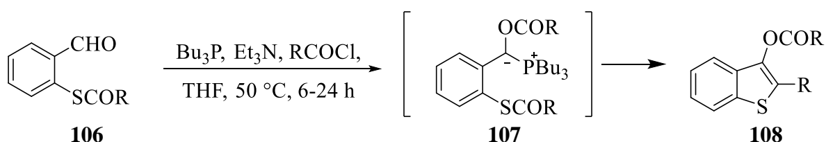
Scheme 29: Intramolecular Wittig reaction of 106 and acid chlorides to yield 108 .
