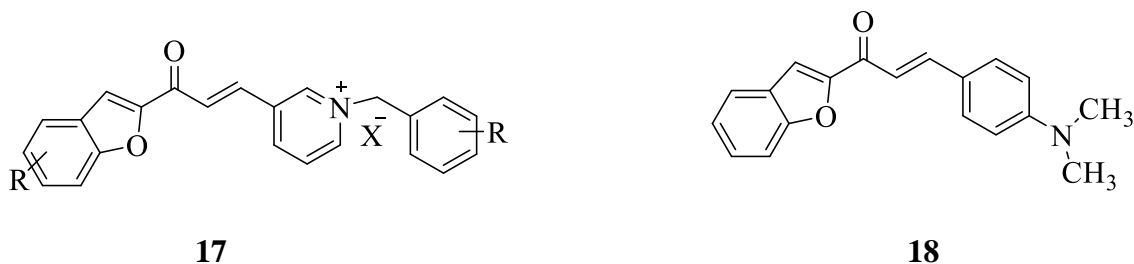
Figure 8: Examples of benzofuran-chalcone hybrids with medicinal applications.
