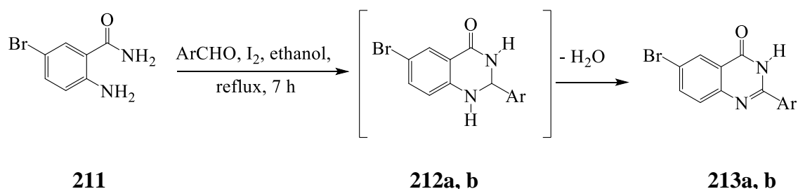
Scheme 65: Iodine-promoted cyclocondensation-dehydrogenation to yield quinazolin-4(3 H )-ones 213
