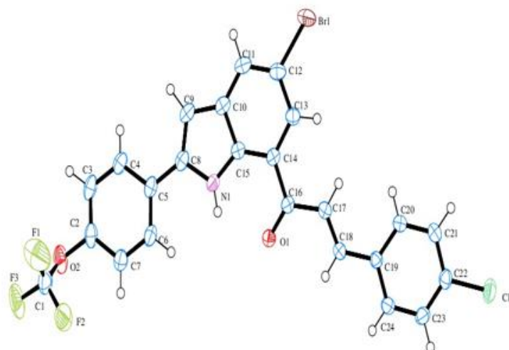
Figure 18: Oak Ridge Thermal Ellipsoid Plot (OTERP) diagram (50% probability level) of compound ( 201e ). H atoms are shown as small spheres of arbitrary size and for clarity they are not labelled.
