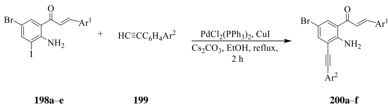
Scheme 58: Sonogashira cross-coupling of 198a-f with terminal acetylenes 199 .
