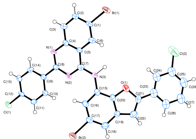
Figure 29: Oak Ridge Thermal Ellipsoid Plot (ORTEP) diagram of 215i . Displacement ellipsoids are drawn at the 50% probability level and H atoms are shown as small spheres of arbitrary radii.
