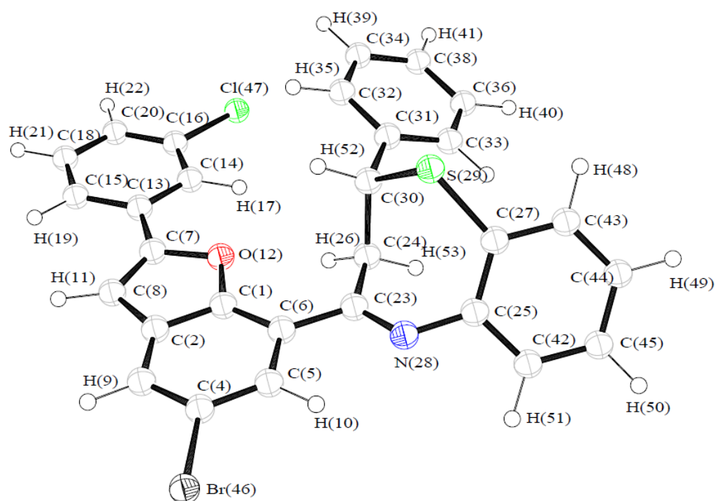
Figure 27: Optimized structure of 205f from DFT calculations.
