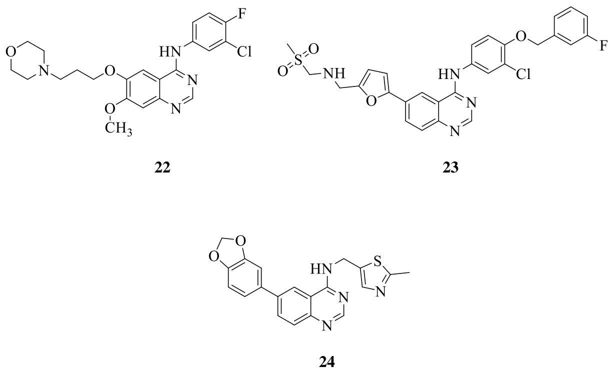
Figure 11: The 4-aminoquinazolines 22–24 with anticancer properties
