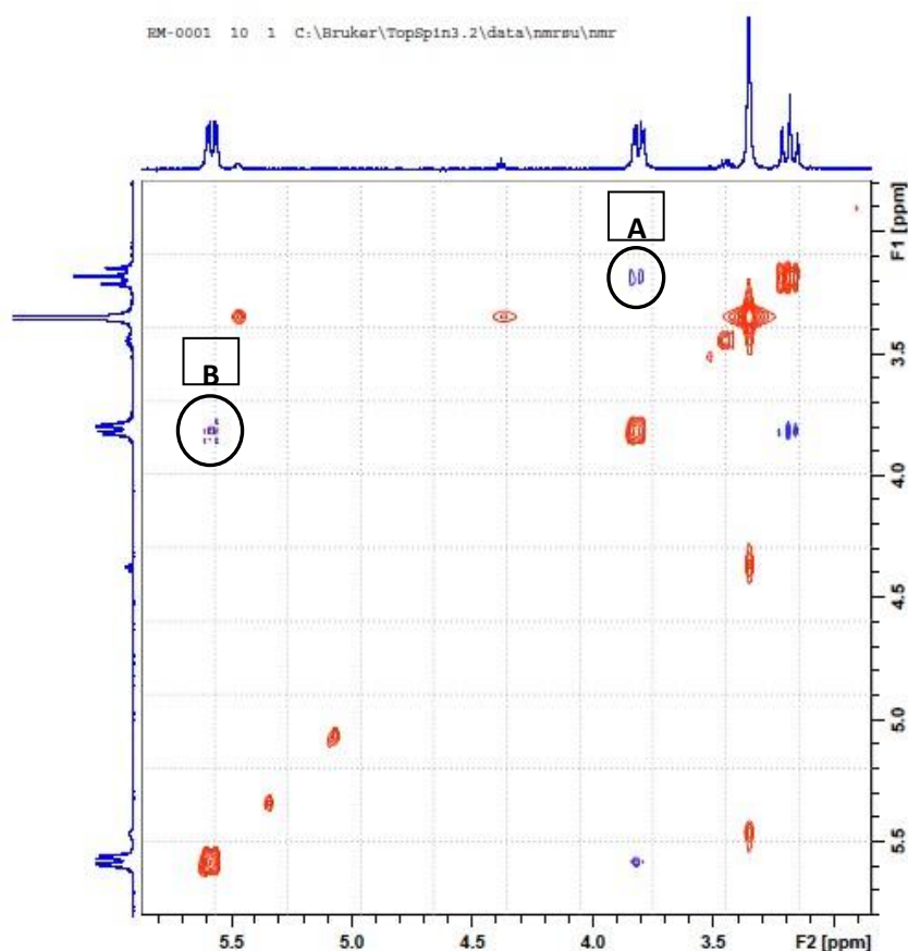
Figure 26: NOESY spectrum of the aliphatic region of compound 205a
