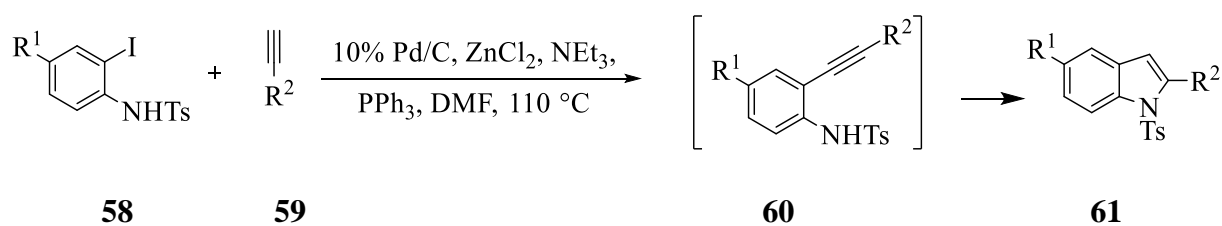
Scheme 11: Synthesis of 2-substituted indoles through annulation promoted by catalytic ZnCl 2 .
