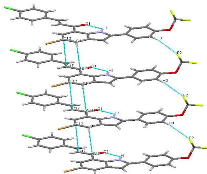
Figure 19: Packing diagram of compound 201e .
