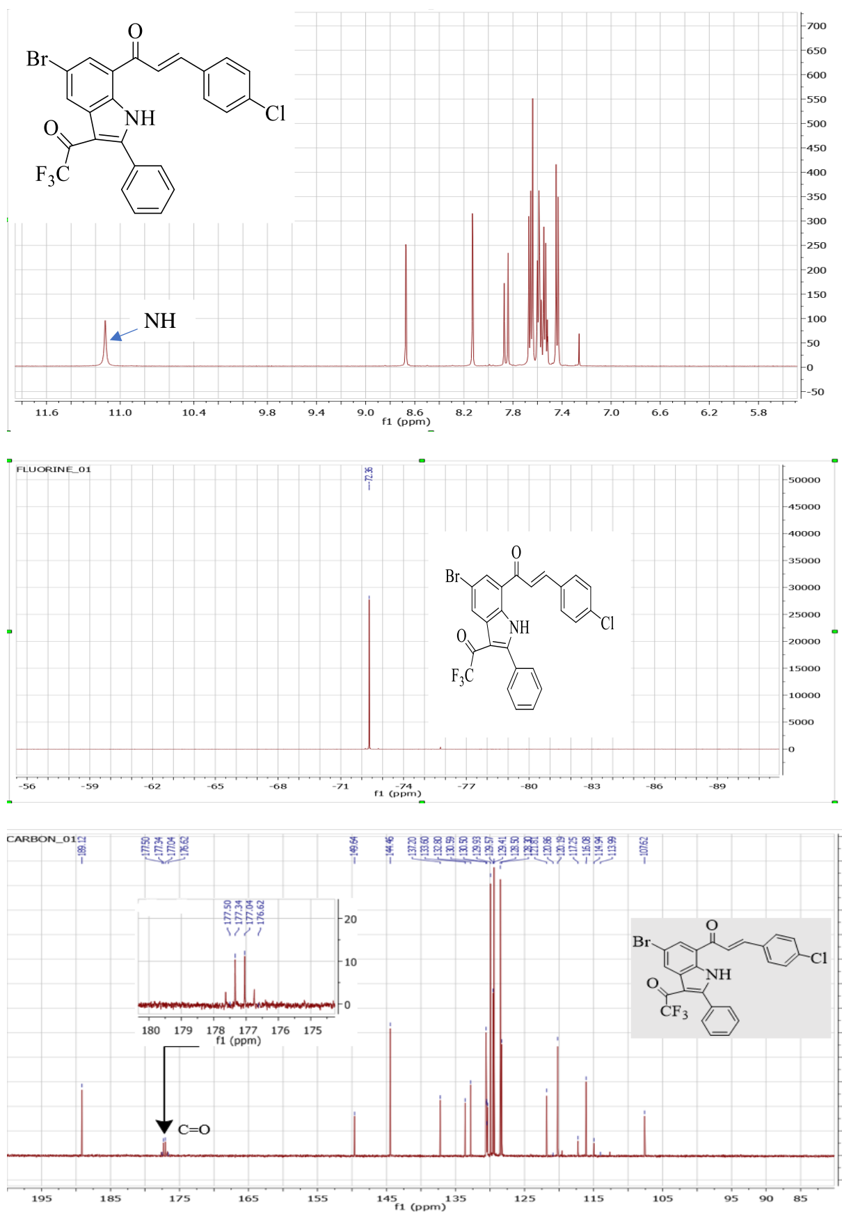
Figure 23: 1 H-, 19 F- and 13 C-NMR spectra of 204d in CDCl 3 at 500 and 125 MHz, respectively.
