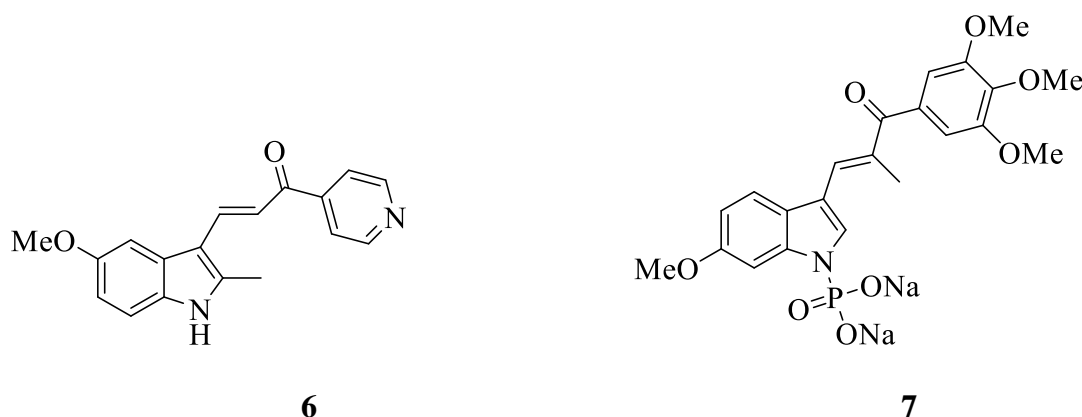
Figure 3: Examples of medicinally important indole-based chalcones.
