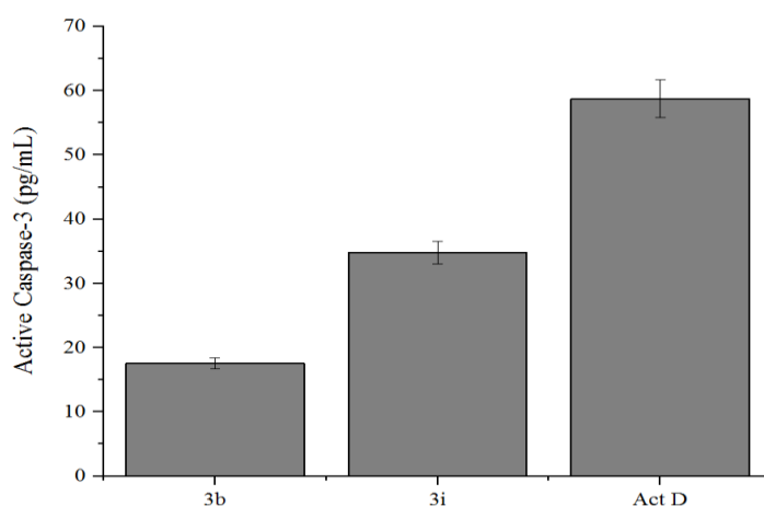
Figure 31. Effects of compounds 203b , 203i , and actinomycin D (Act. D) at 1 \mu M on human Caspase-3 (Asp175) activity in MCF-7 cells, respectively.
