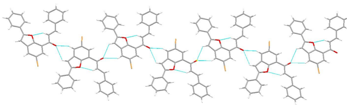
Figure 22: Packing diagram of 203a showing the 1D ribbon
