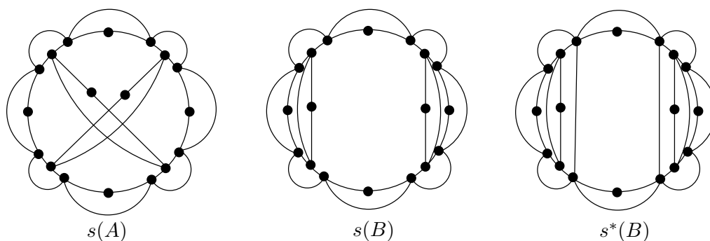
Figure 4.22: Graphs s(A) , s(B) and s^*(B)
